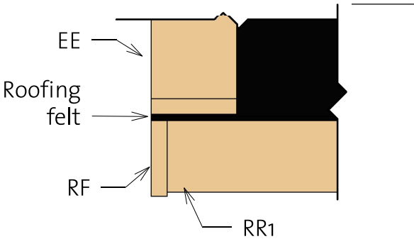
3 Roof Reinforcement
